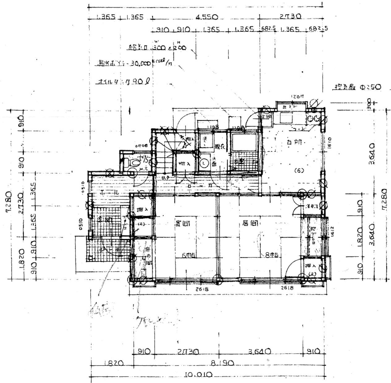
1ST.FLOOR
